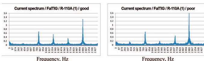
Fig. 5. a. Current spectrum. Electrode: Omnia 46 Weldability: good. Source: FalTig 200. Current: 110A; b. Current spectrum. Electrode: Omnia 46 Weldability: poor. Source: FalTig 200. Current: 110A
