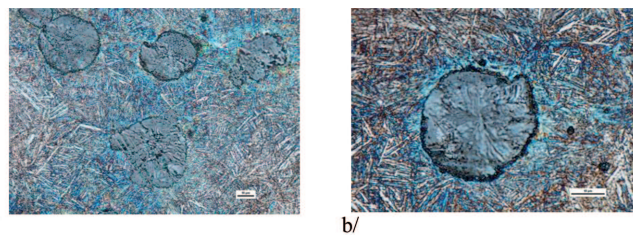
Fig. 7. Structure of ADI – EN-GJS-1200-2, after 10.400 thermal fatigue cycles, a – zone of heating to 500^{\circ}\text{C} , b – zone of heating to 250 \div 300^{\circ}\text{C} – magnification 500x, etched by nital
