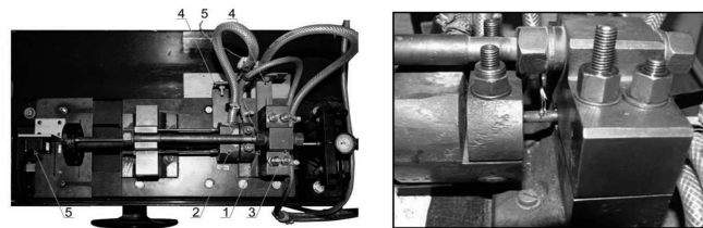
Fig. 2. System of fixing samples in the stand for testing thermal fatigue: a – View from above ( 1-sample, 2-mobile jaw, 3-master jaw, 4-feeders, 5-laser sensor of displacing, 6-thermo-couple; b - View of the fixed sample [5,8÷12,14÷16]
