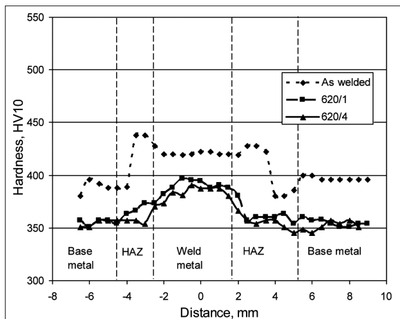
Fig. 16. Distribution of hardness vs. distance after welding and aging 620°C/1h, 620°C/4h
