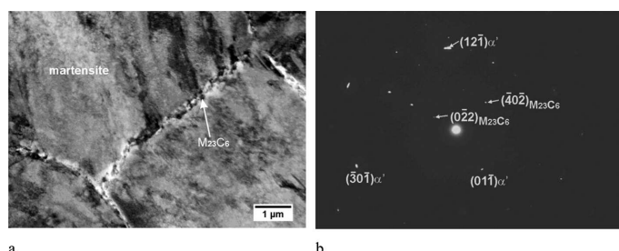
Fig. 9. Weld microstructure after annealing 620°C / 1 hour, b) electron diffraction pattern, [\bar{1}22]M_{23}C_6 , [\bar{1}23]_{\alpha}
