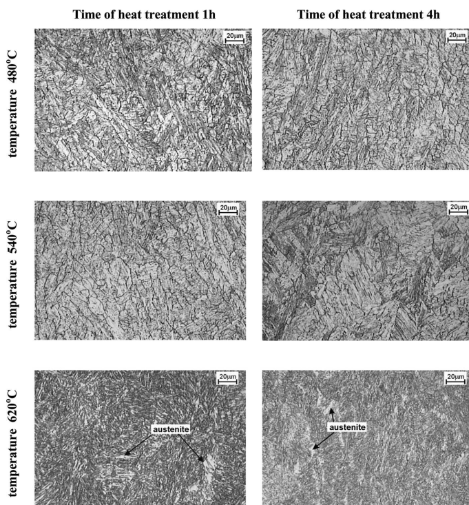
Fig. 8. Weld metal microstructure after heat treatment
