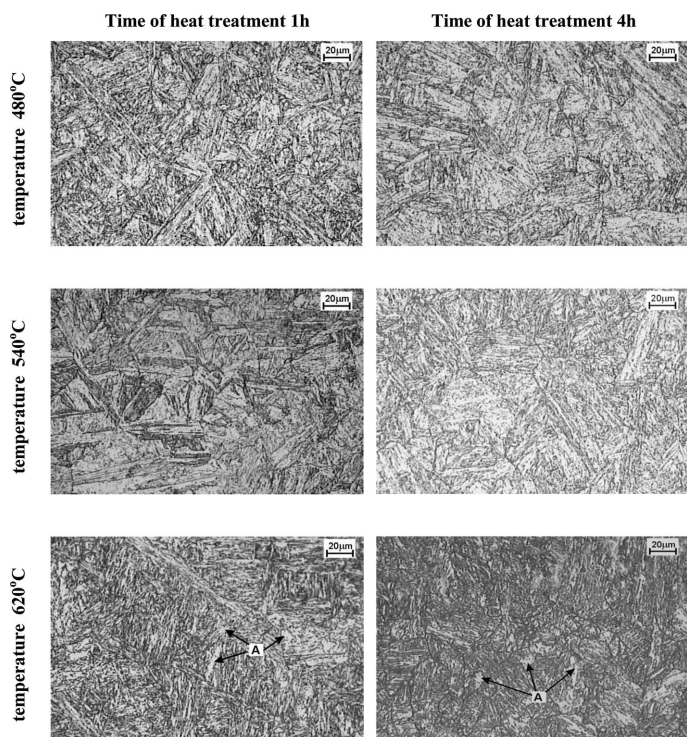
Fig. 6. Base metal microstructure after heat treatment. The bright regions visible between the plater of austenite (marked by arrows and capital letter "A")
