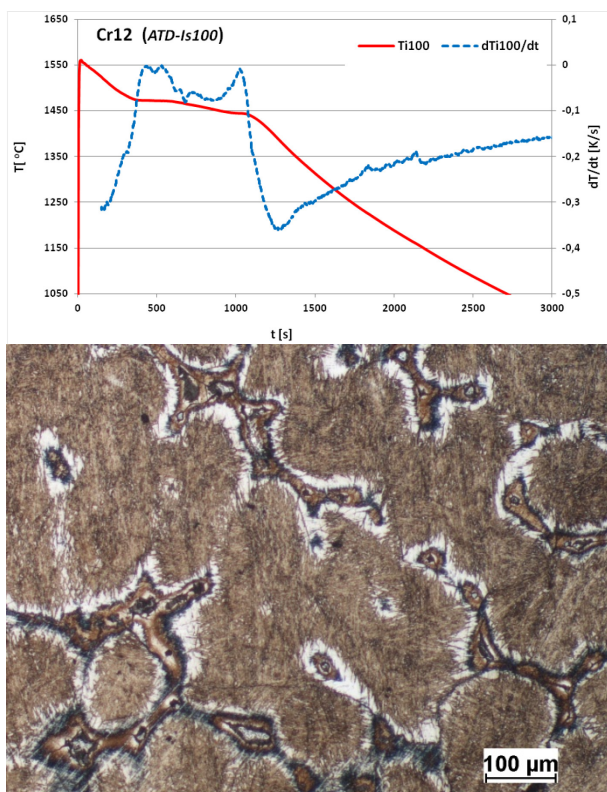
Fig.6. TDA curves and structures of examined cast steels – specimen casting with the highest solidification module ( M=2,50 )
