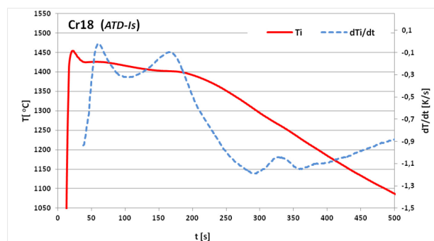
Fig. 5. TDA curves of examined cast steels – specimen casting with moderate solidification module ( M=0,90 )
