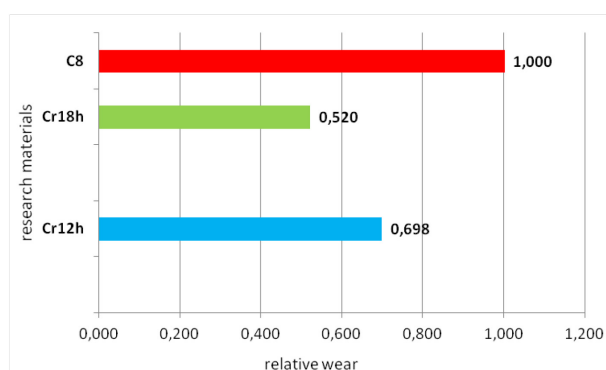
Fig. 9. Relative wear of Cr-Ni-Mo cast steel
