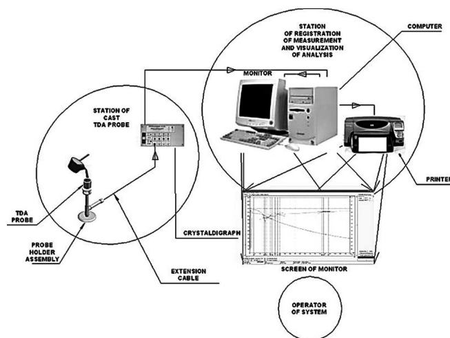
Fig. 3. Scheme of the TDA measuring station
