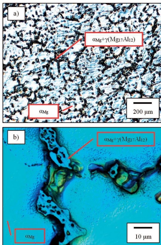
Fig. 5. Microstructure of the AM60 alloy solidifying in the ceramic TDA sampler
