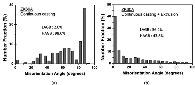
Fig. 2. Distributions of the number fractions of the grain boundary misorientation angles for the ZK60A alloy after (a) continuous casting and (b) extrusion
