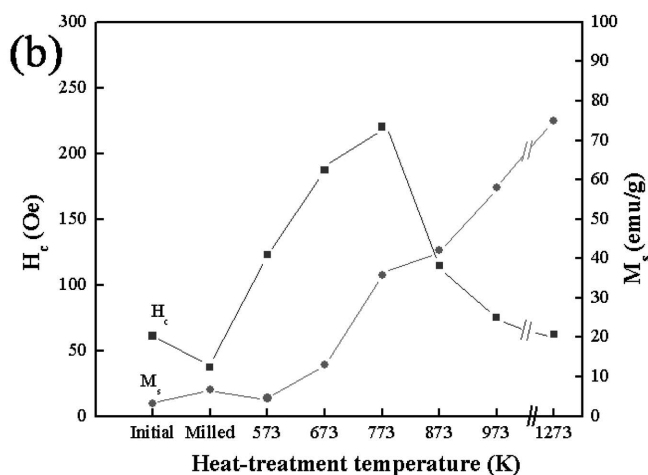
Fig. 7. M-H loops (a) and coercivity ( H_c ) and saturation magnetization ( M_s ) (b) of the initial, milled and heat-treated ferrite powders
