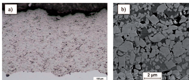
Fig. 9. Microstructure of the coating cross section deposited from a mixture of WC-Co 83-17 standard powder and \text{Cr}_3\text{C}_2
