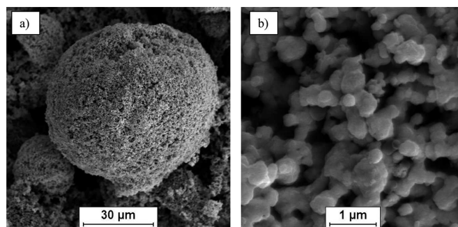
Fig. 4. SEM image of WC powder, a) agglomerate, b) particles
