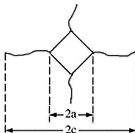
Fig. 1. Schematic of the Vickers indentation used for the fracture toughness determination
