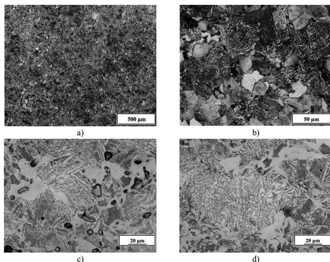
Fig. 2. The characteristic microstructures of DH-1 PM steel after SAT 500 variant (a, b – Leica DM4000M; c, d) – Leica DM LM
