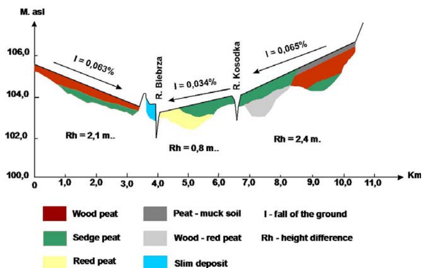
Fig. 6. Cross-section no. 14
