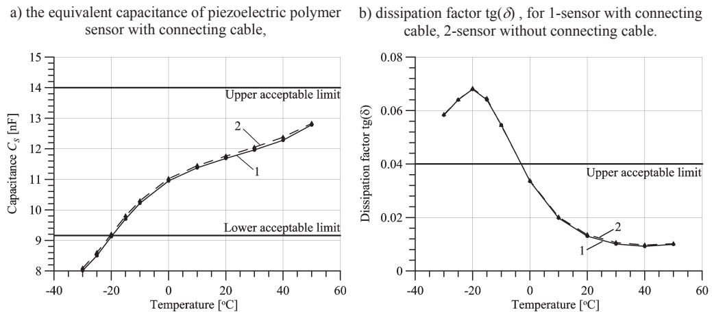
Fig. 8. The influence of temperature on:
