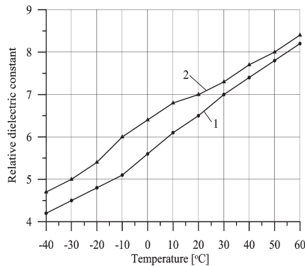
Fig. 5. Dielectric constant of piezoelectric polymer sensors' material versus temperature; measurement results at the frequency of : 1 - 1kHz, 2 - 10kHz.
