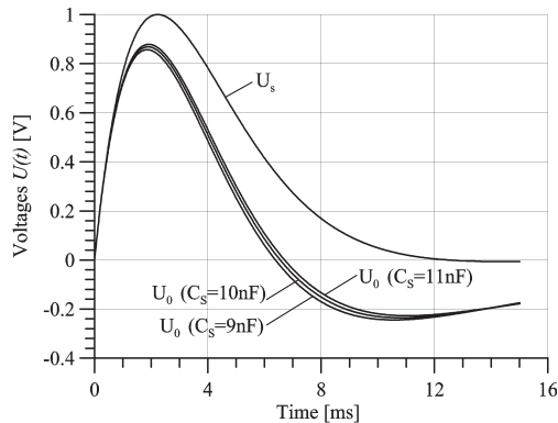
Fig. 3. Exemplary waveforms of the load signal from piezoelectric polymer sensor.
