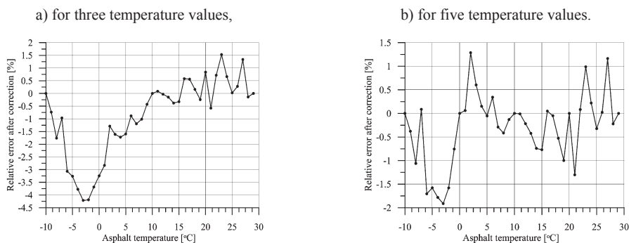
Fig. 12. The relative error of weighing in the WIM system after correction based on calibration:
