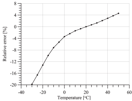
Fig. 9. The weighing error in the WIM system equipped with piezoelectric polymer sensors, arising exclusively from a change in the sensor parameters due to a change in temperature.
