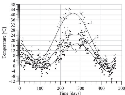
Fig. 6. Changes in the pavement temperature in the south of Poland during a 16-month period. 1 – maximum daily temperature, 2 – average daily temperature, 3 – minimum daily temperature.
