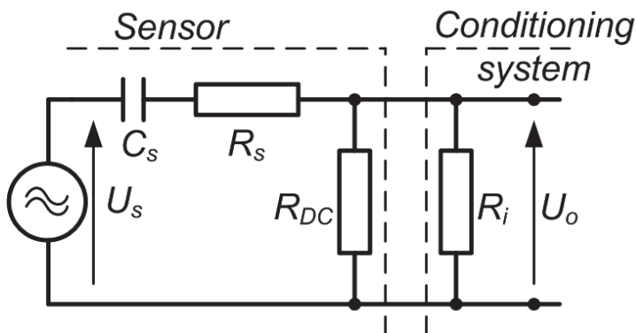
Fig. 4. The equivalent circuit (model) of a piezoelectric polymer sensor and the input part of conditioning system waveforms of the load signal from piezoelectric polymer sensor.
