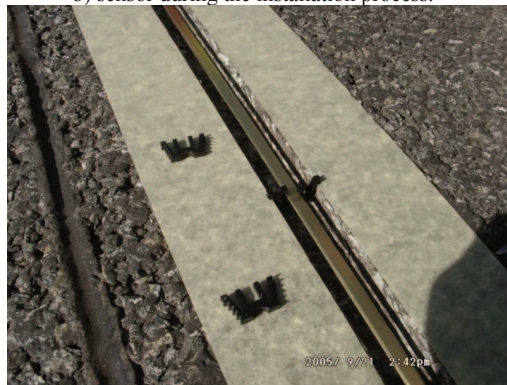
b) sensor during the installation process.
