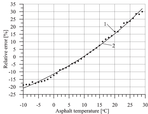
Fig. 10. The relative error of weighing a reference vehicle at different temperatures on WIM site installed in asphalt. 1 – experimental results, 2 – the model characteristic.
