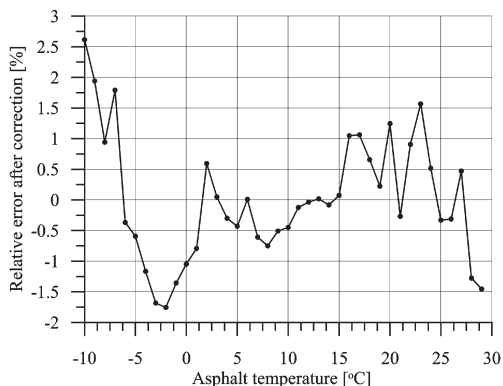
Fig. 11. The relative error of weighing in the WIM system after correction based on the model (4).
