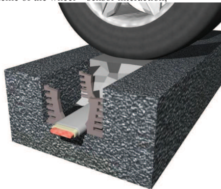
a) scheme of the wheel – sensor interaction,
