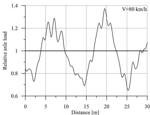
Fig. 1. Relative changes in the vehicle instantaneous axle load at the speed of 80 km/h.
