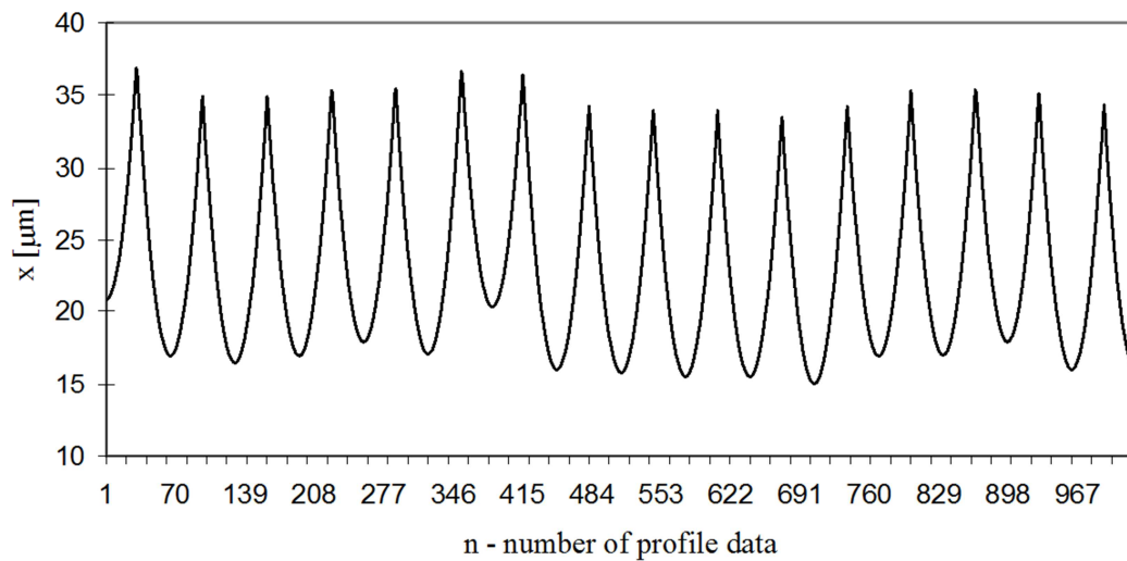
Fig. 8. Generated irregularity course with curved tool profile with disturbances of perpendicular displacements of the tool against the workpiece, sampling interval h = 4 \mu\text{m} .
