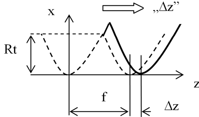
Fig. 3. Transversal irregularities with displacement of the tool edge outline parallel to the workpiece's axis "Δz".
