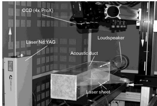
Fig. 4. Experimental setup with PIV measurement system.
