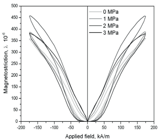
Fig. 4 Magnetostrictive dependence of the magnetic field intensity of the composite materials with the polyurethane matrix reinforced with 20% volume fraction of the Tb_{0.3}Dy_{0.7}Fe_{1.9} powder with granulation A
