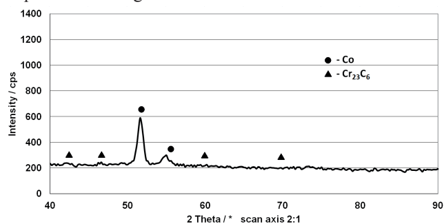
Fig. 6. X- ray diffraction of alloy No. 27
