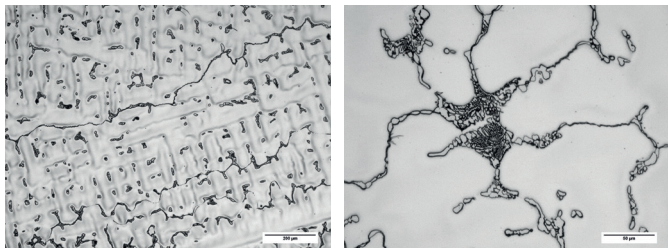
Fig. 3. Microstructure of alloy No. 28
