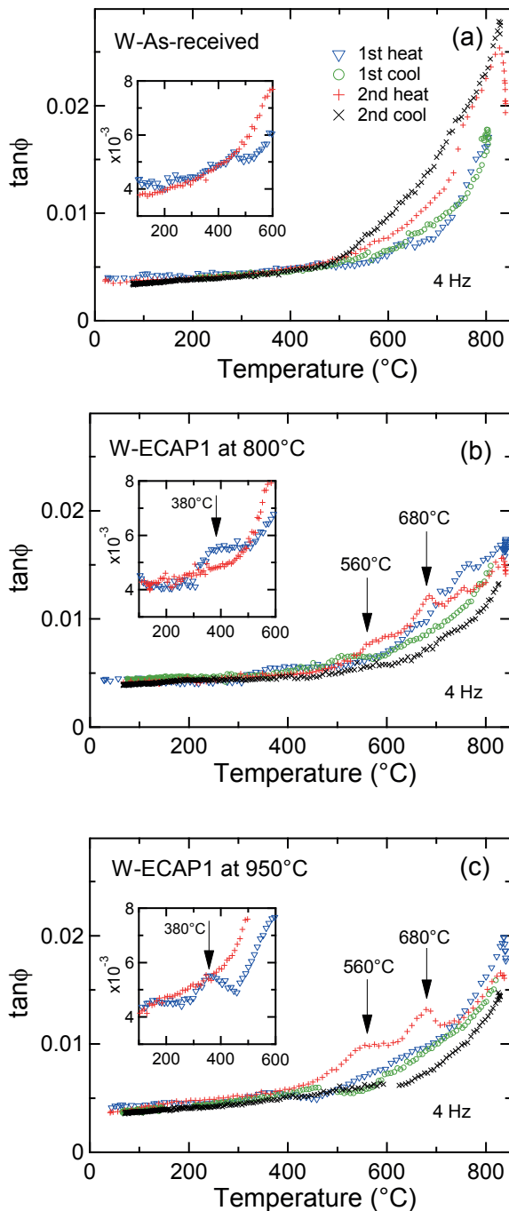
Fig. 4. Internal friction peaks in two heating-cooling cycles in: (a) as-received W, (b) 1 pass at 800°C strained W, (c) 1 pass at 950°C strained W; inset: a small peak at 380°C
