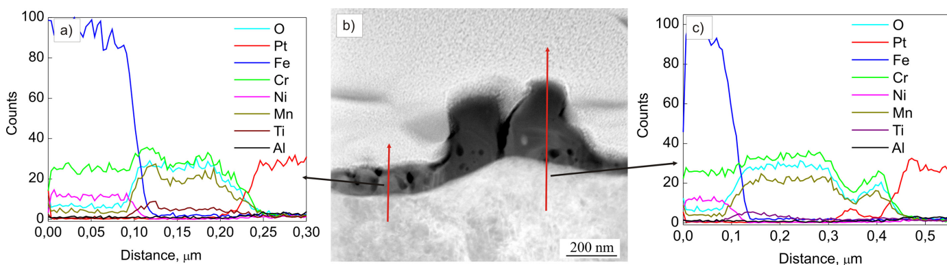
Fig. 9. The HAADF/STEM image presenting the structure of oxides and the analysis of TEM with EDS chemical composition on cross-section of the oxidized layer formed on the AISI 321 steel in a vacuum furnace with graphite heating chamber
