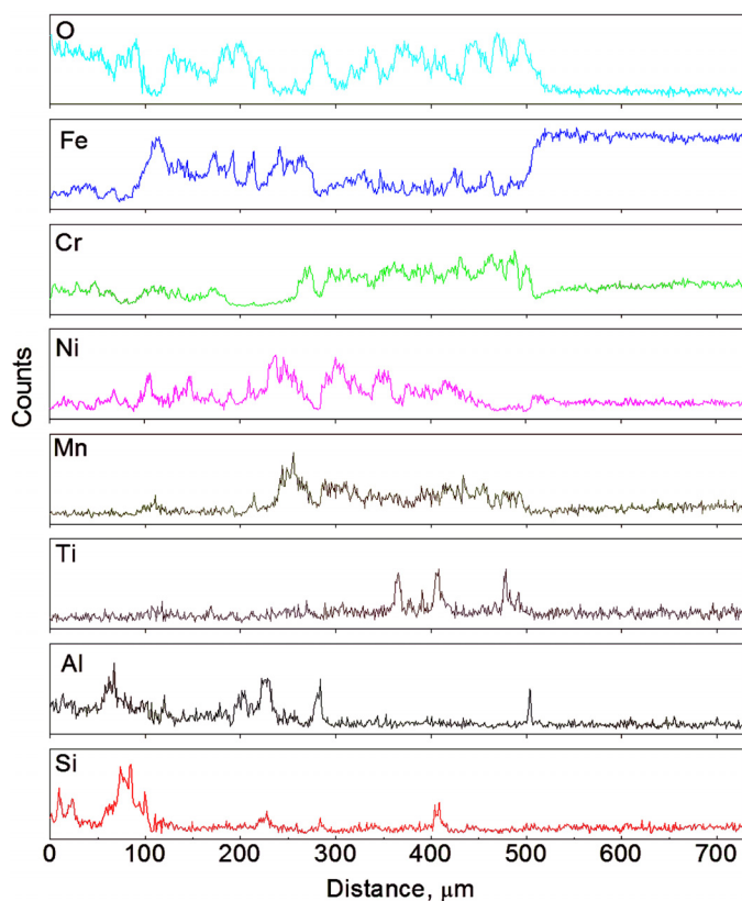
Fig. 4. EDS chemical composition change along the indicated A line on the Fig. 5b
