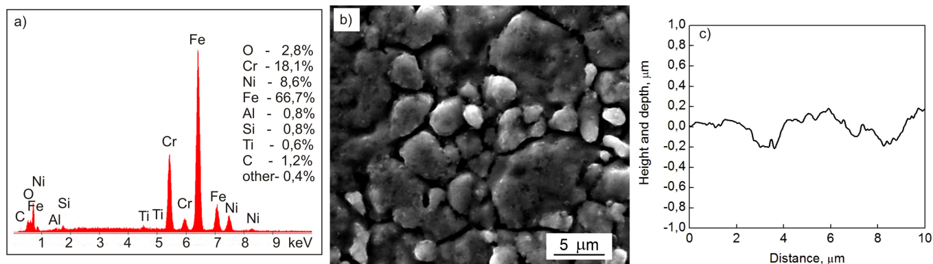
Fig. 7. The microstructure of the oxidized layer of the AISI 321 steel as a result of annealing in a vacuum furnace with molybdenum heating chamber: a) EDS spectrum and chemical composition (wt.%) of the surface in Fig. b., b) microstructure of the surface of oxides, c) profiles of the oxide layer surface
