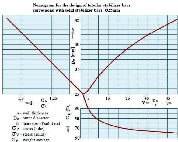
Fig. 1. Nomogram for the design of tubular stabilizer bars correspond with solid stabilizer bars Ø25 mm [1–6, 9]
