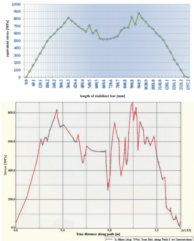
Fig. 14. Equivalent stresses: a) analytical calculations, b) tension curve created with HyperWorks (FEM)
