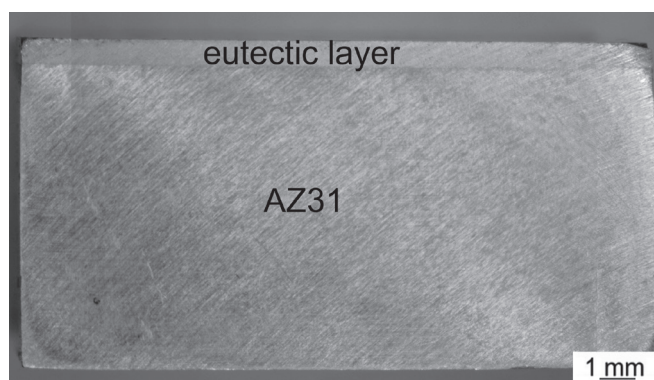
Fig. 2. The AZ31/eutectic specimen with an eutectic layer thickness of 1100 \mu\text{m} , fabricated by the thermochemical treatment method
