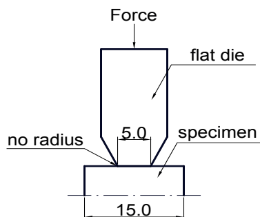
Fig. 3. The schedule of the rectangular prism specimen compression test using the Gleeble 3800 simulator
