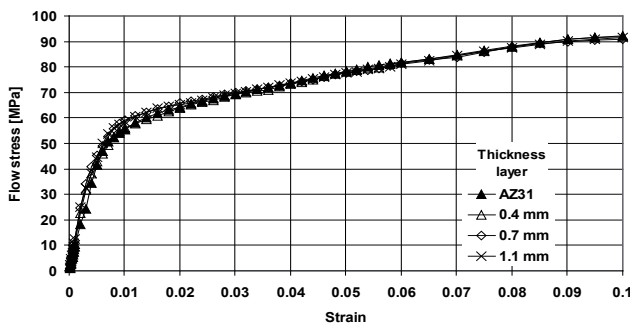
Fig. 7. The plastic flow curves obtained from the compression testing of two-layered AZ31/eutectic specimens and an AZ31 magnesium alloy specimen at a temperature of 420°C and a strain rate of 1 \text{s}^{-1}
