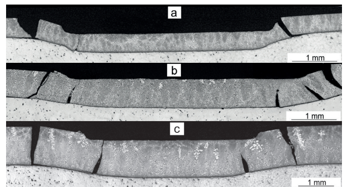
Fig. 8. Two-layered AZ31/eutectic specimens with varying eutectic layer thickness after the compression test at a temperature of 420°C (strain rate, 1 \text{s}^{-1} ; deformation, 0.1): a) 400 \mu\text{m} , b) 700 \mu\text{m} , c) 1100 \mu\text{m}
