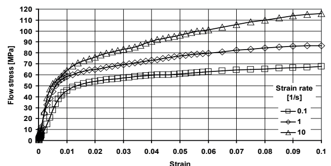
Fig. 9. The plastic flow curves obtained from the compression tests of two-layered AZ31/eutectic specimens with an eutectic layer thickness of 700 \mu\text{m} for different strain rates
