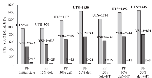
Fig. 5. The results of the mechanical properties of PF samples in the initial state, after deformation of 15, 30 and 50% and heat treatment
