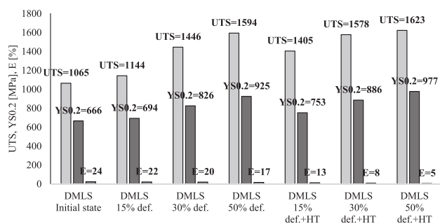
Fig. 6. The results of the mechanical properties of DMLS samples in the initial state, after deformation of 15, 30 and 50% and heat treatment
