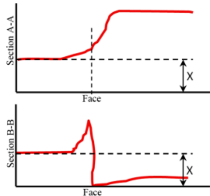
Fig. 3. Abutment pressures distribution for sections A-A and B-B of Figure 2; X shows the average of in-situ stress
