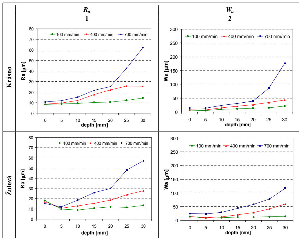
Changes of the R_a and W_a for 3 studied rocks and for 3 water jet cutting speed
