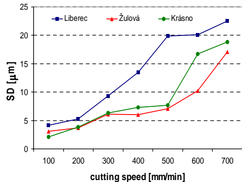
Fig. 8. The standard deviation of the mean R_a for the whole areas
