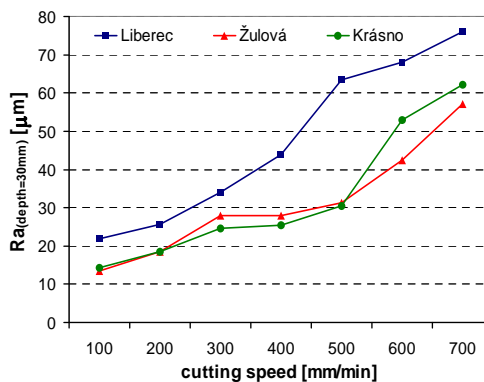
Fig. 6. R_a determined at a depth of 30 mm
