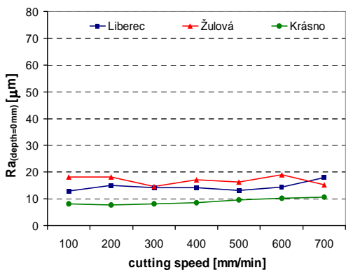
Fig. 5. R_a determined at a depth of 0 mm
