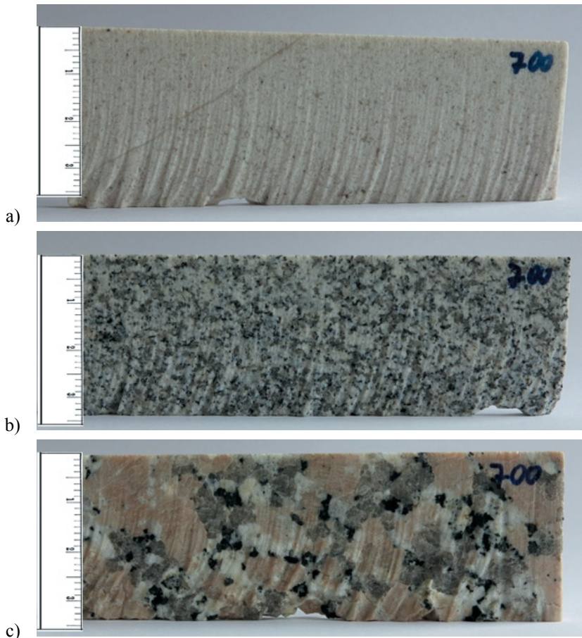
Fig. 4. Examples of surface samples cut at a speed of 700 \text{ mm}\cdot\text{min}^{-1} . (a) the fine-grained granite from Krásno, (b) the medium-grained granite from Žulová, (c) the coarse-grained granite from Liberec. The height of the samples = c.a. 32 mm
