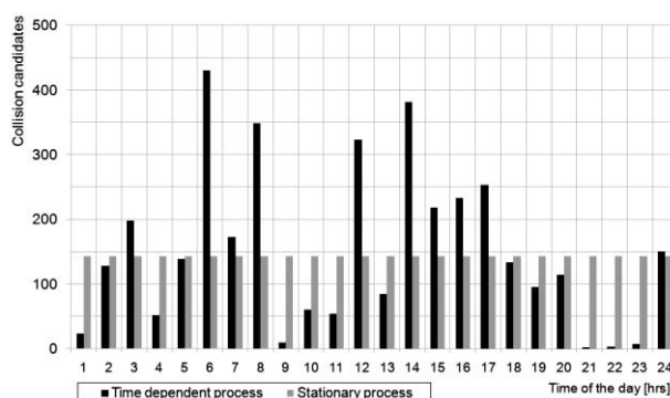
Fig. 5. A number of collision candidates obtained from the MDTC model for constant and time varying traffic flows
