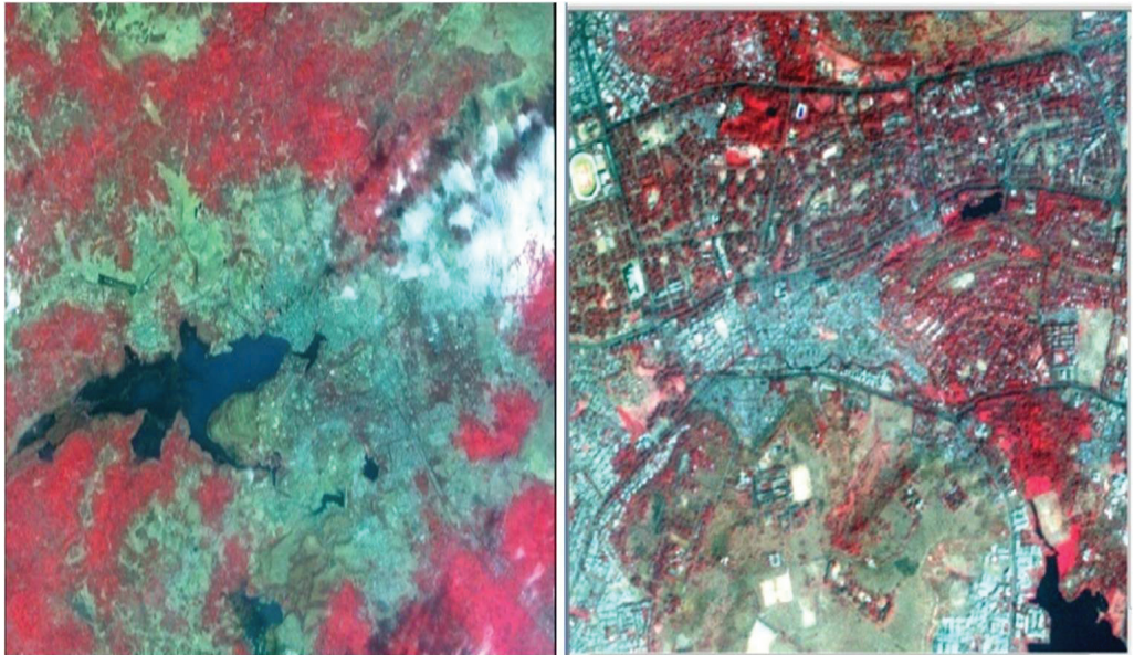
a) FCC of Bhopal observed by LISS-IV sensor
